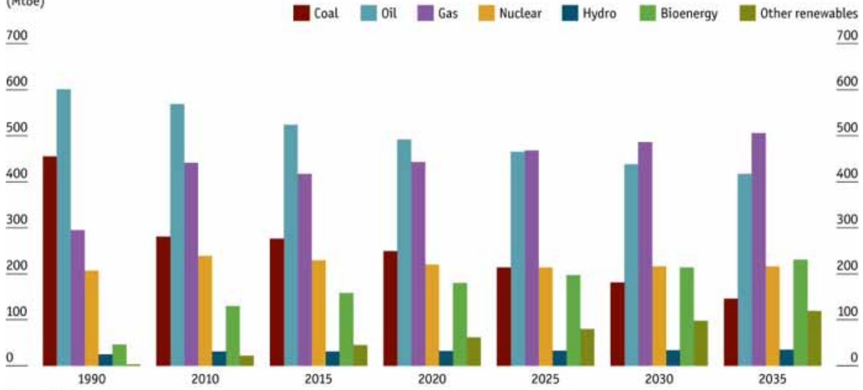
Total primary energy demand in the EU (Mtoe)
