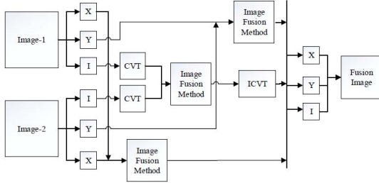
Fig. 5. The steps in the proposed image fusion algorithms
